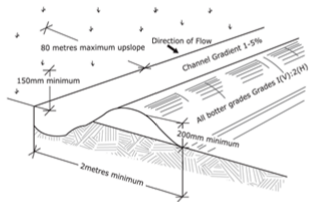
Note: Only to be used as temporary bank where maximum upslope length is 80metres
