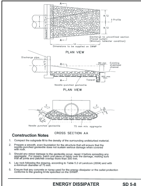
ENERGY DISSIPATOR
