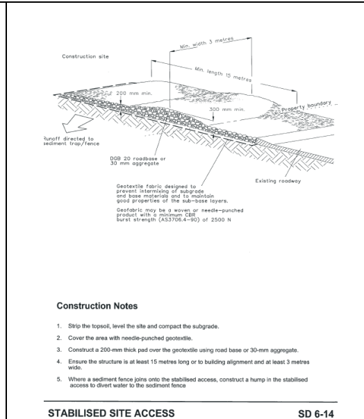
STABILISED SITE ACCESS
