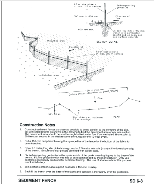
SEDIMENT FENCE
