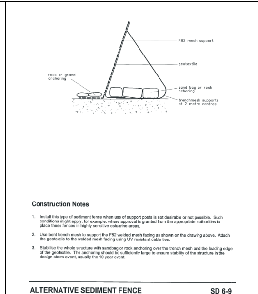
ALTERNATIVE SEDIMENT FENCE
